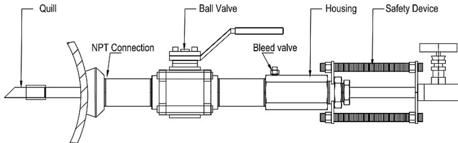
Pic. 5.c. Retractable Sampling System
