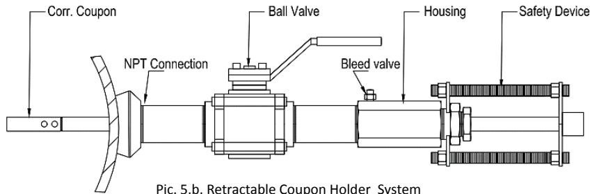
Pic. 5.b. Retractable Coupon Holder System
