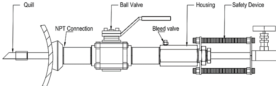
Pic. 5.d. Retractable Chemical Injection System
