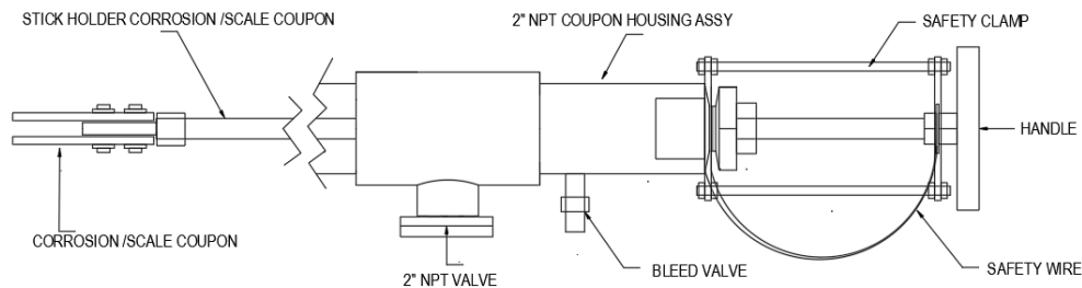
Pic. 5.e. Retractable Stick Coupon Holder
