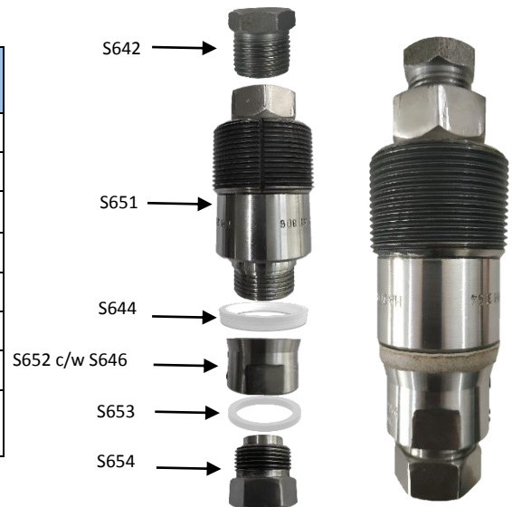
Pic. 6.g. Hollow Plug Assy.
